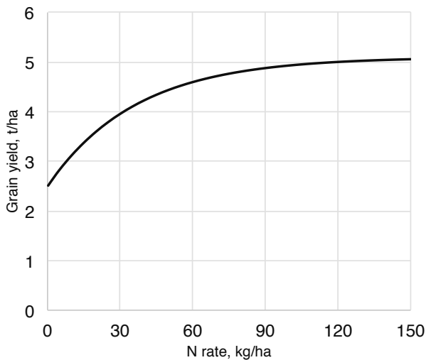
Figure 9.4: A curvilinear yield response maize to applied N for the Highland AEZ of Malawi ( Y = 5.1 - 2.6 * 0.973^N ).
